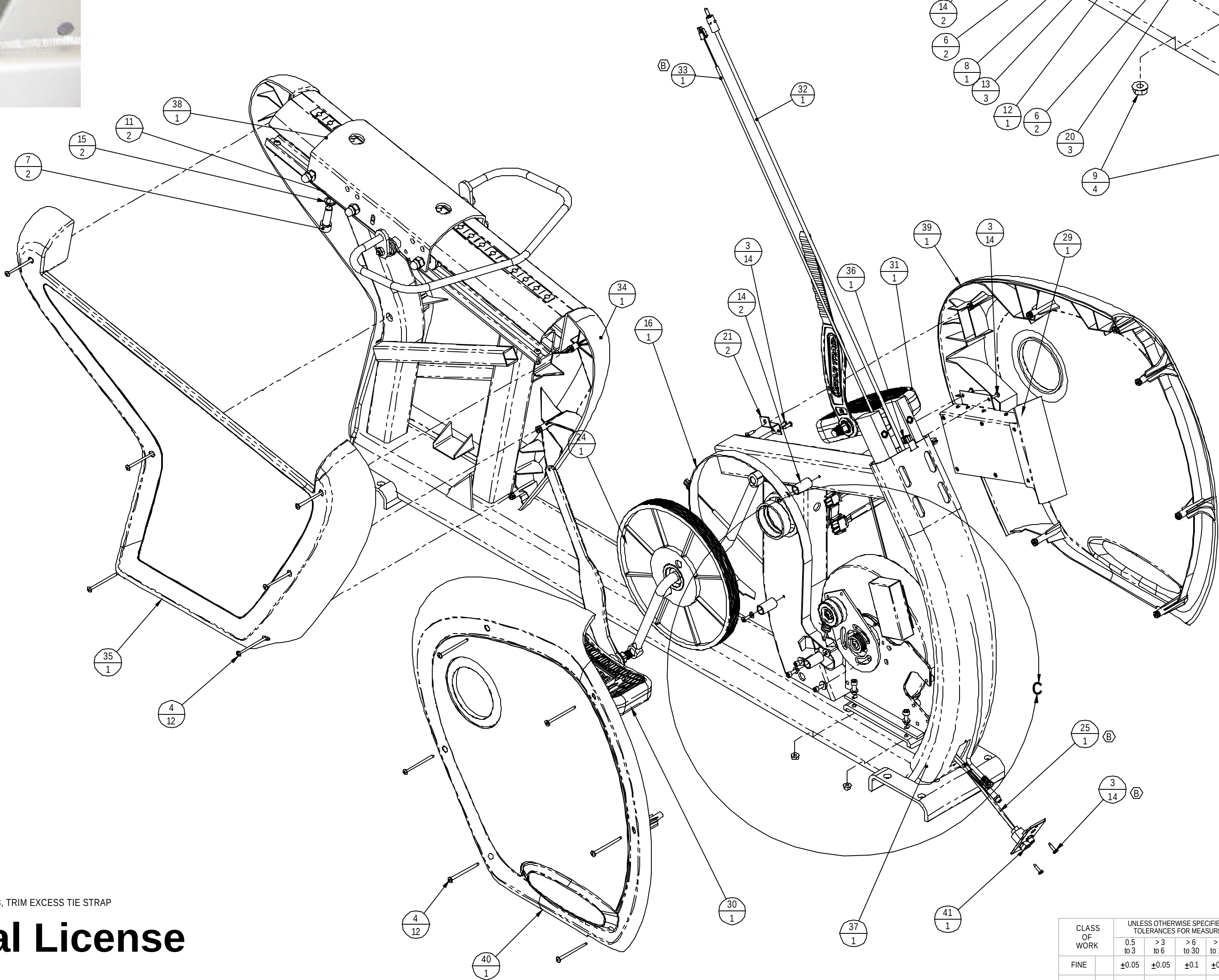
DETAIL C SCALE 2 : 5
